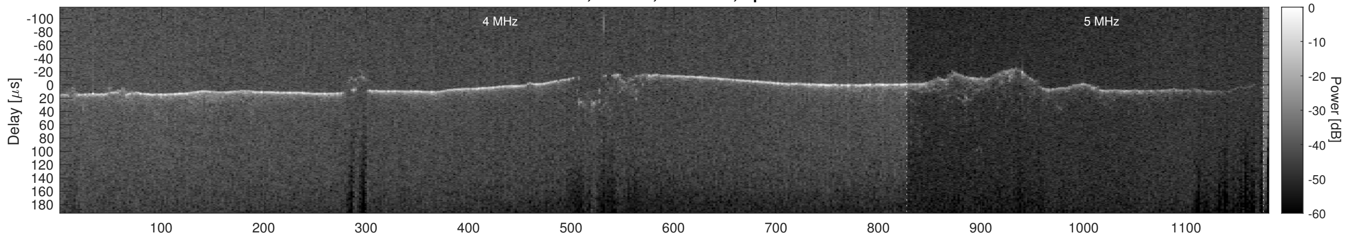
Orbit 9200, Cluttergram
