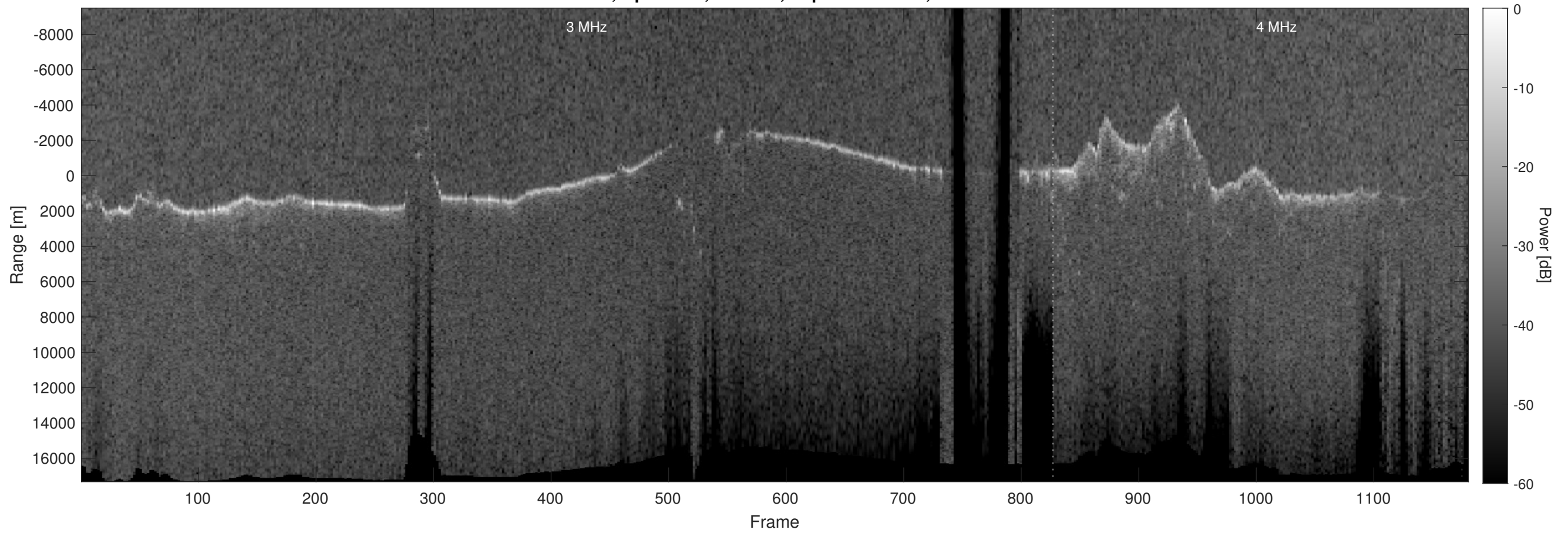
Orbit 9200, Optimized, Window, Depth-Corrected, Channel 2
