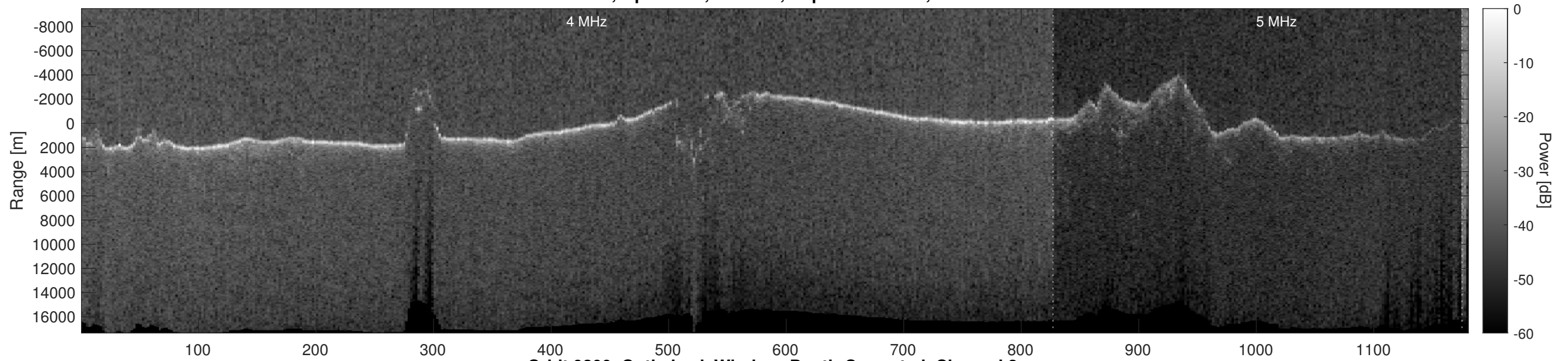
Orbit 9200, Optimized, Window, Depth-Corrected, Channel 2
