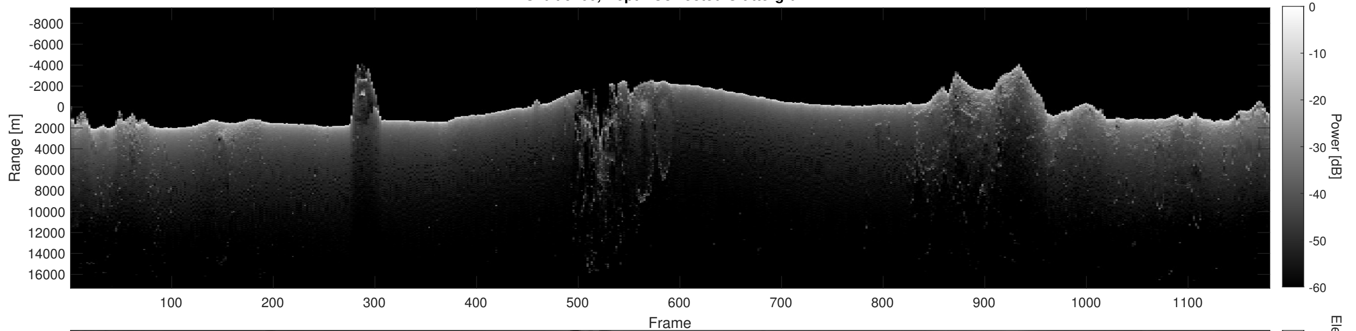
Orbit 9200, Depth-Corrected Cluttergram
