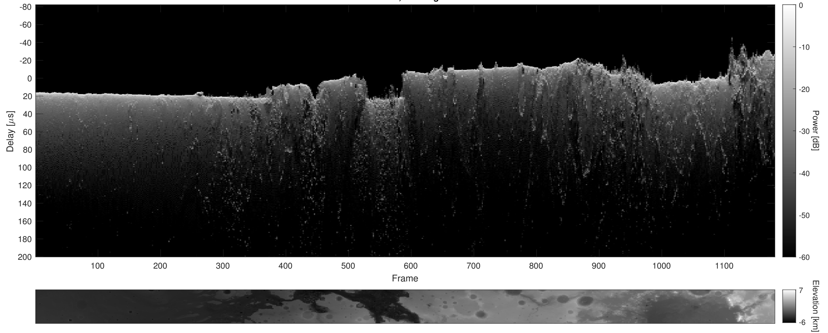
Orbit 9203, Cluttergram
