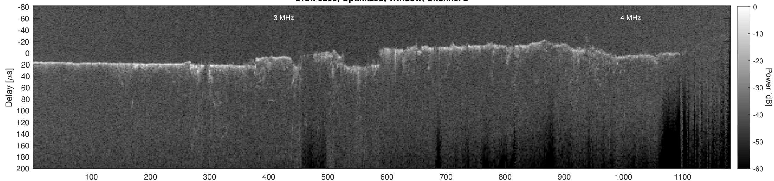
Orbit 9203, Cluttergram
