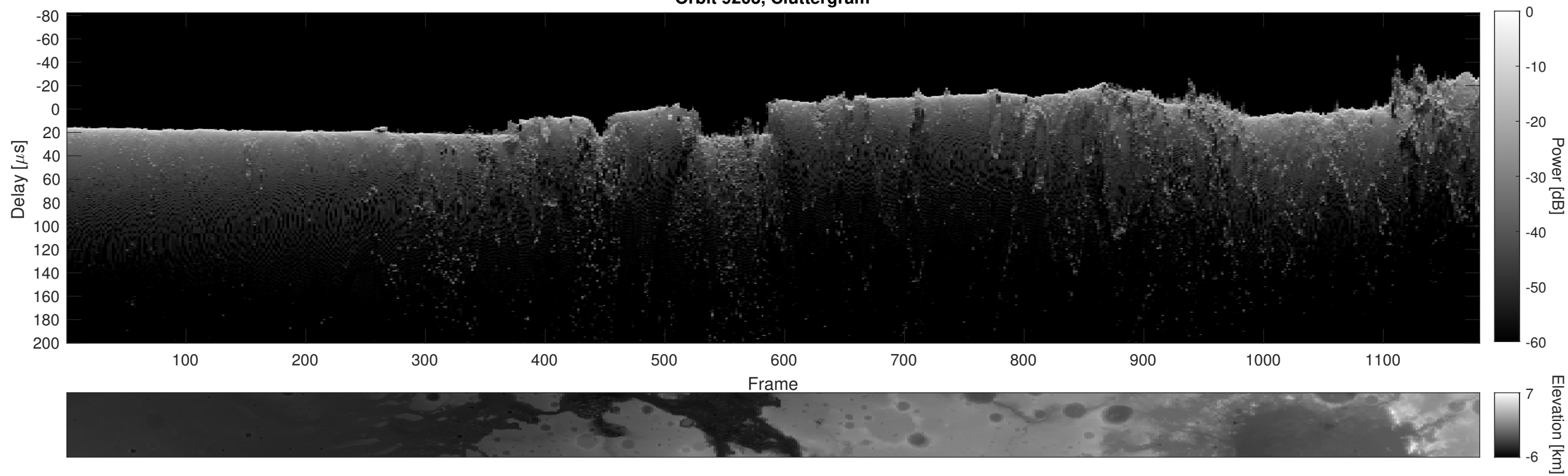
Orbit 9203, Cluttergram
