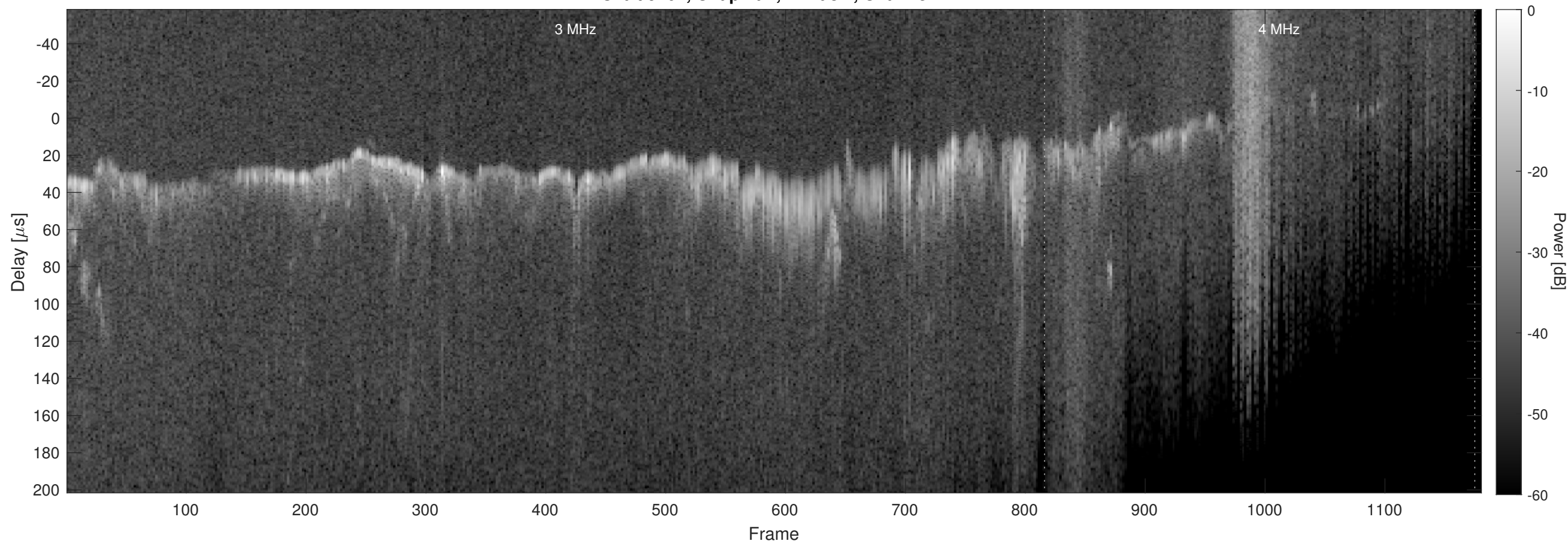
Orbit 9204, Chapman, Window, Channel 2
