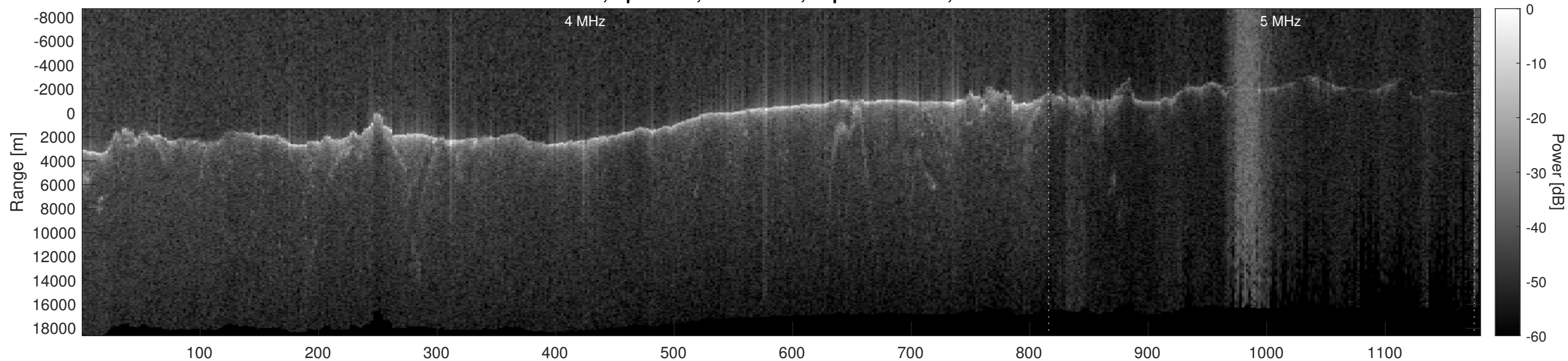
Orbit 9204, Optimized, No Window, Depth-Corrected, Channel 2
