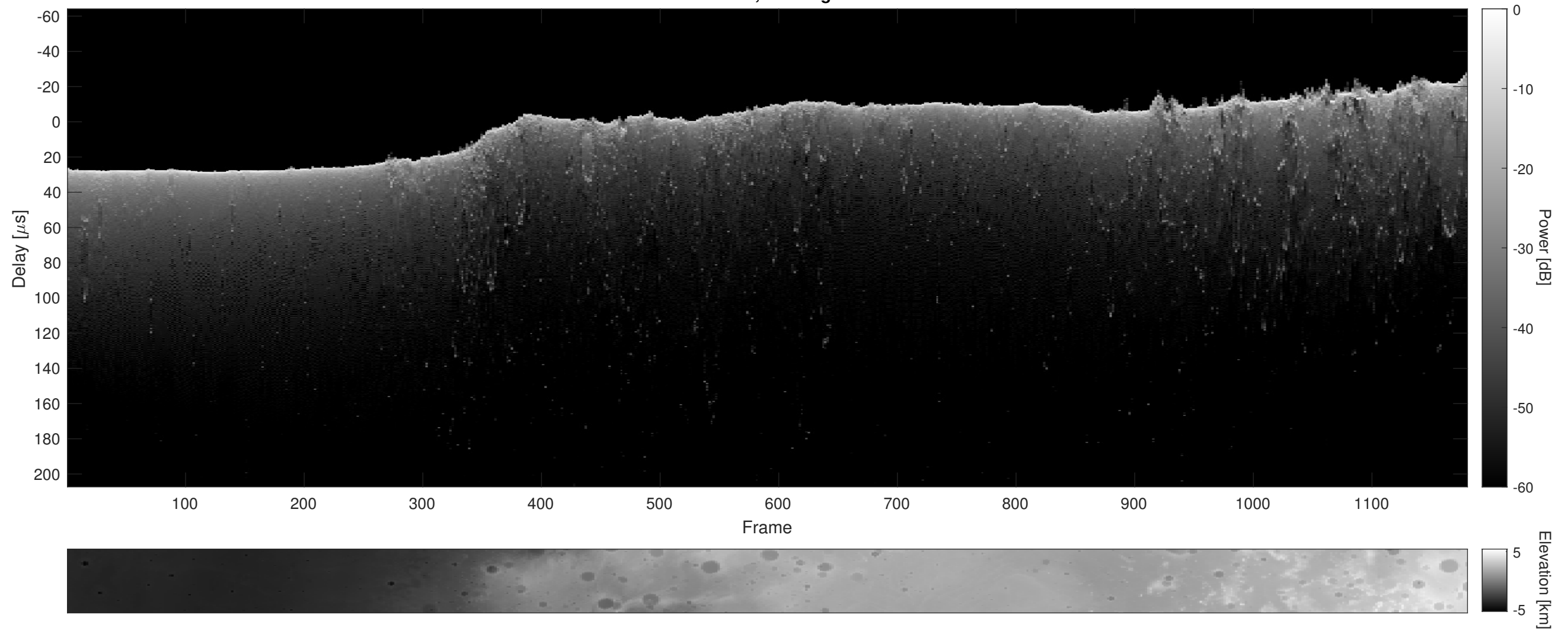
Orbit 9205, Cluttergram
