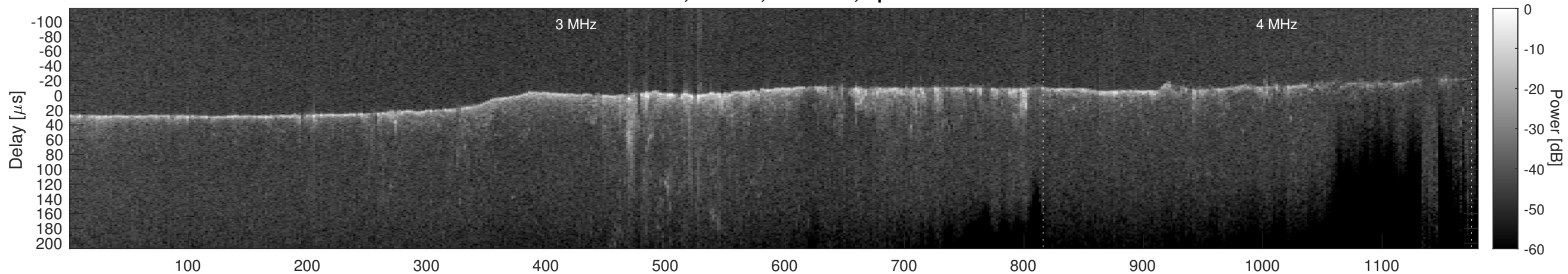
Orbit 9205, Cluttergram
