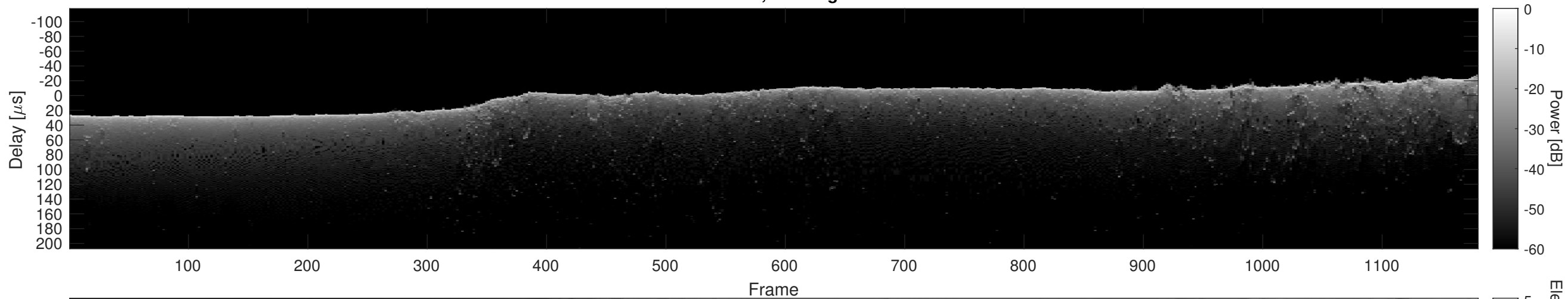
Orbit 9205, Cluttergram
