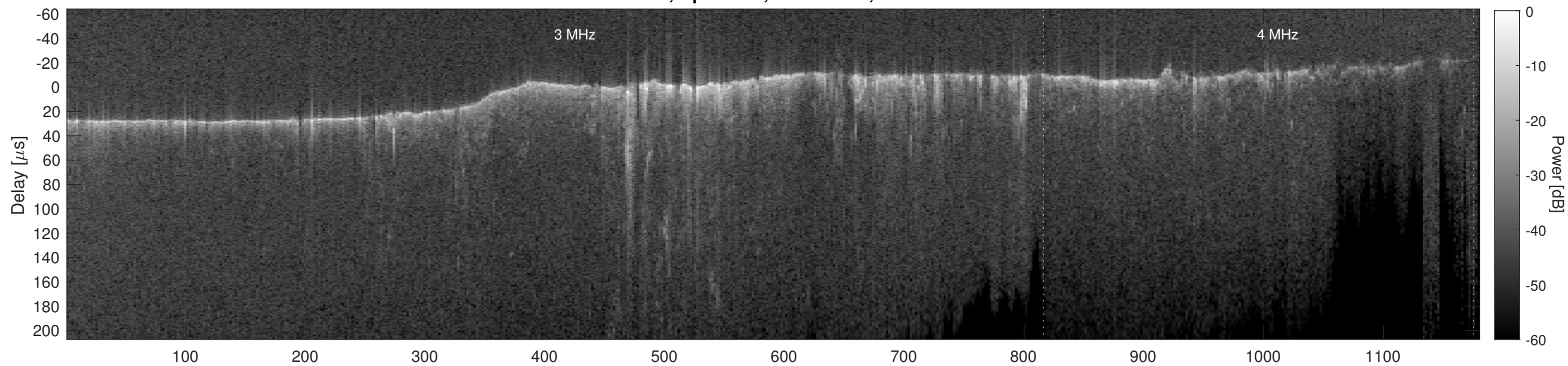
Orbit 9205, Cluttergram
