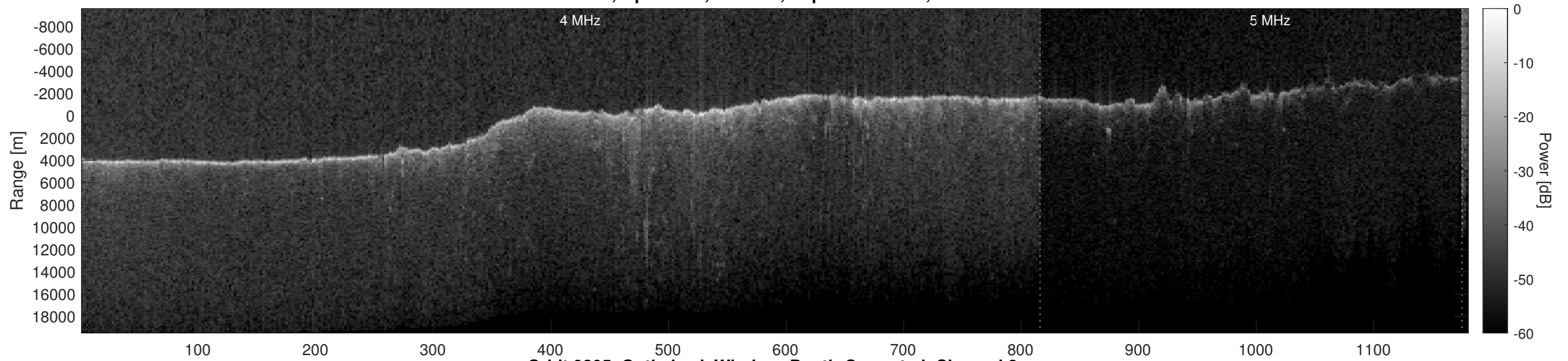
Orbit 9205, Optimized, Window, Depth-Corrected, Channel 2
