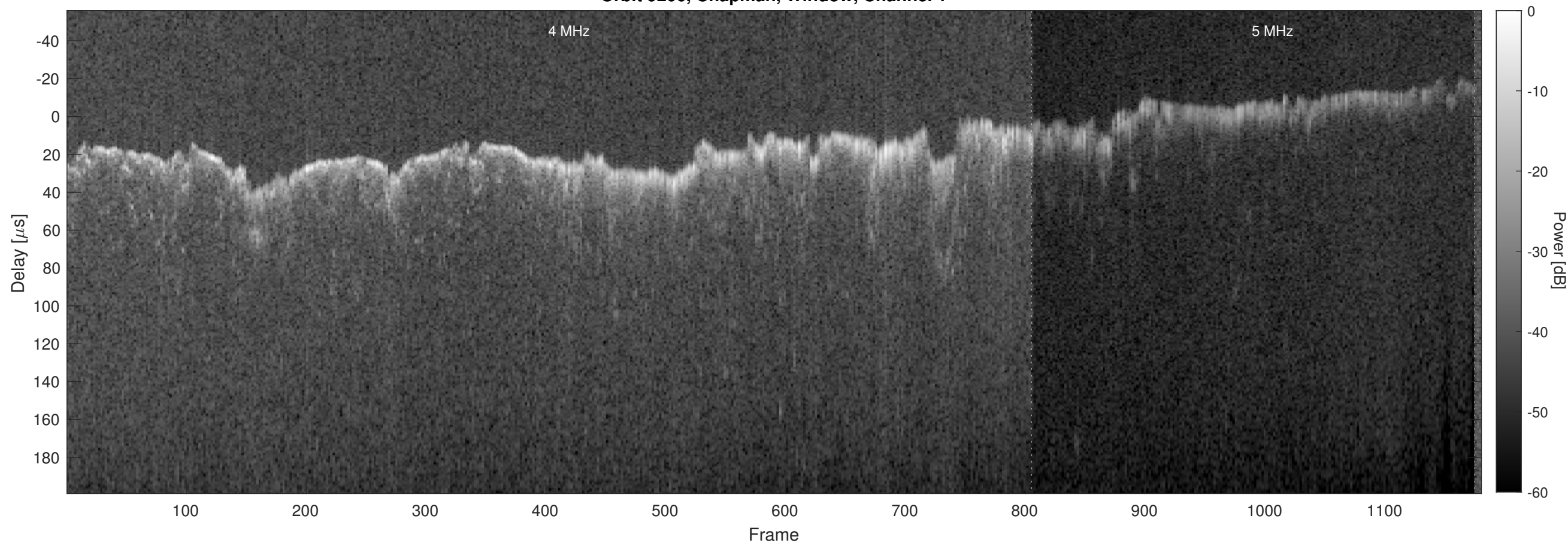
Orbit 9206, Chapman, Window, Channel 2
