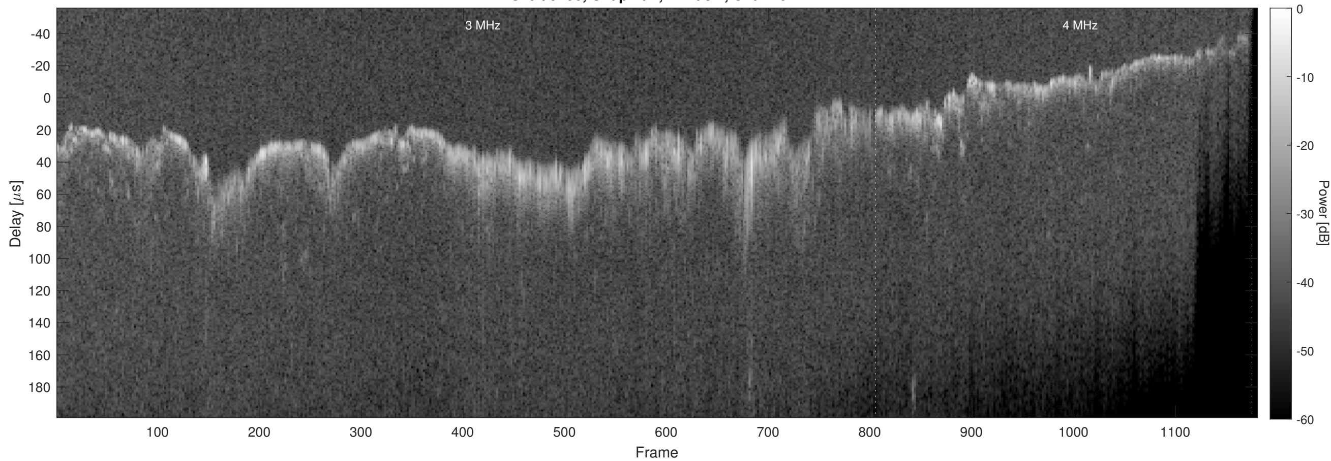
Orbit 9206, Chapman, Window, Channel 2
