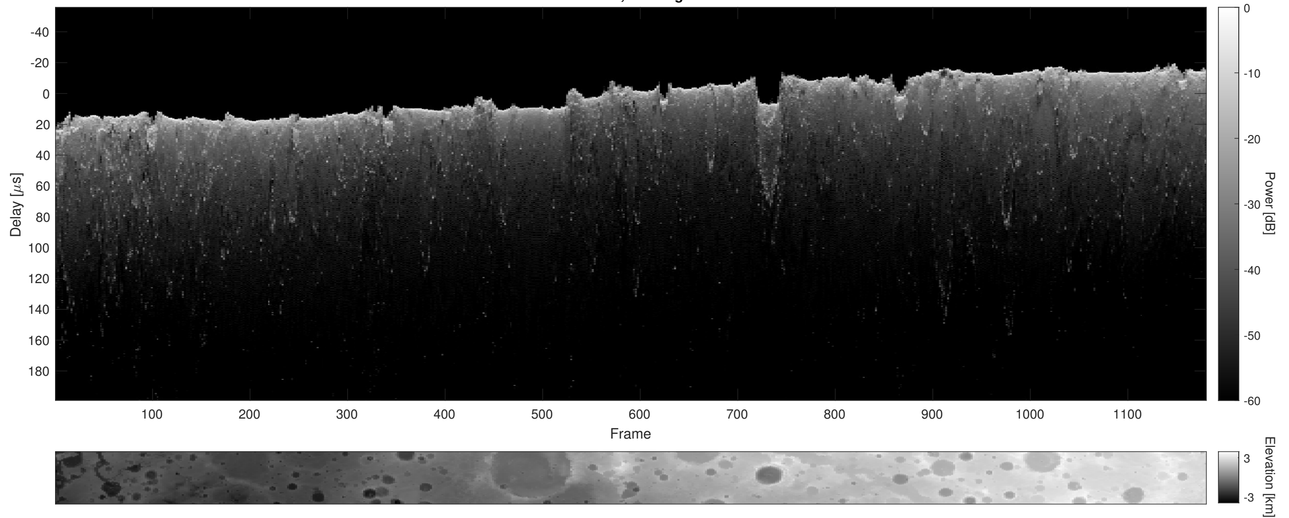
Orbit 9206, Cluttergram
