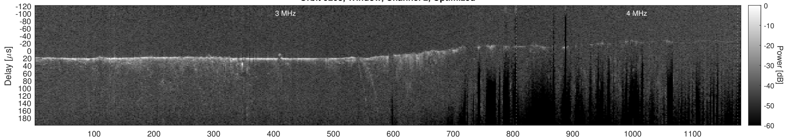
Orbit 9208, Cluttergram
