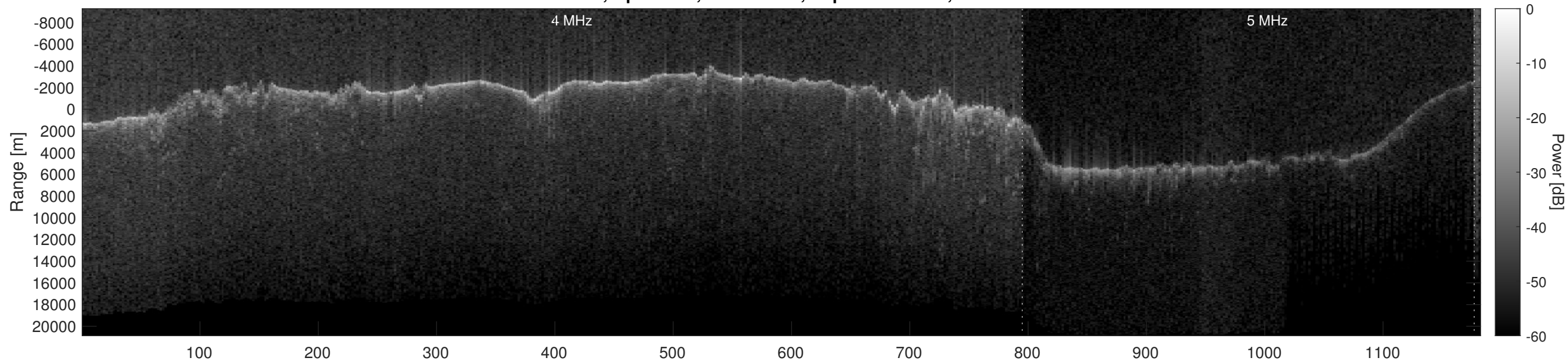
Orbit 9209, Optimized, No Window, Depth-Corrected, Channel 2
