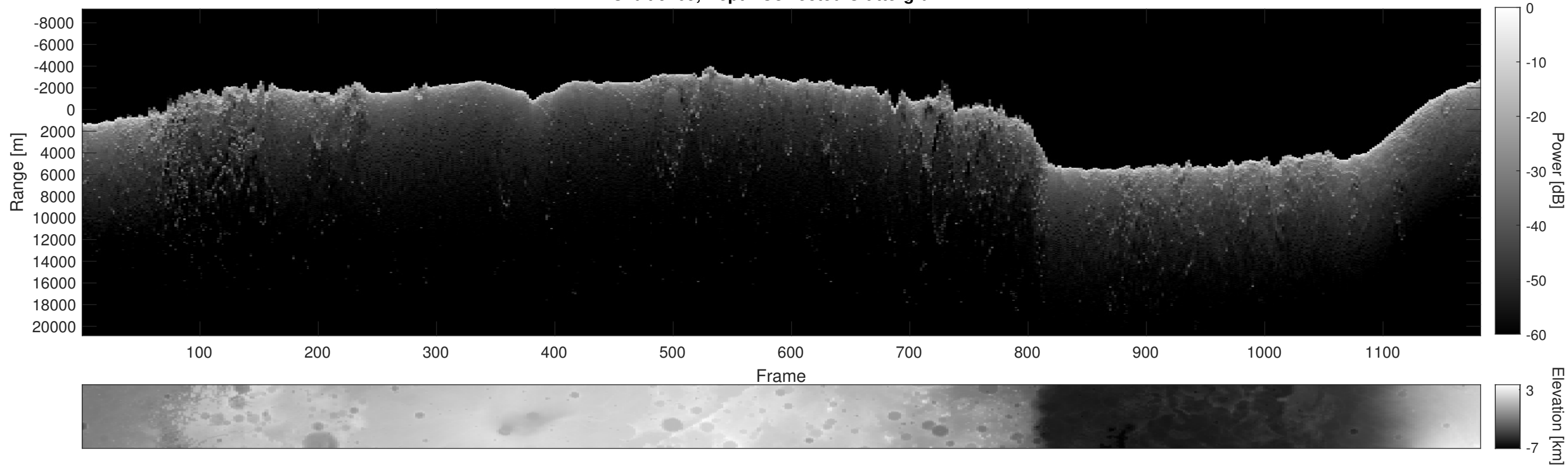
Orbit 9209, Depth-Corrected Cluttergram
