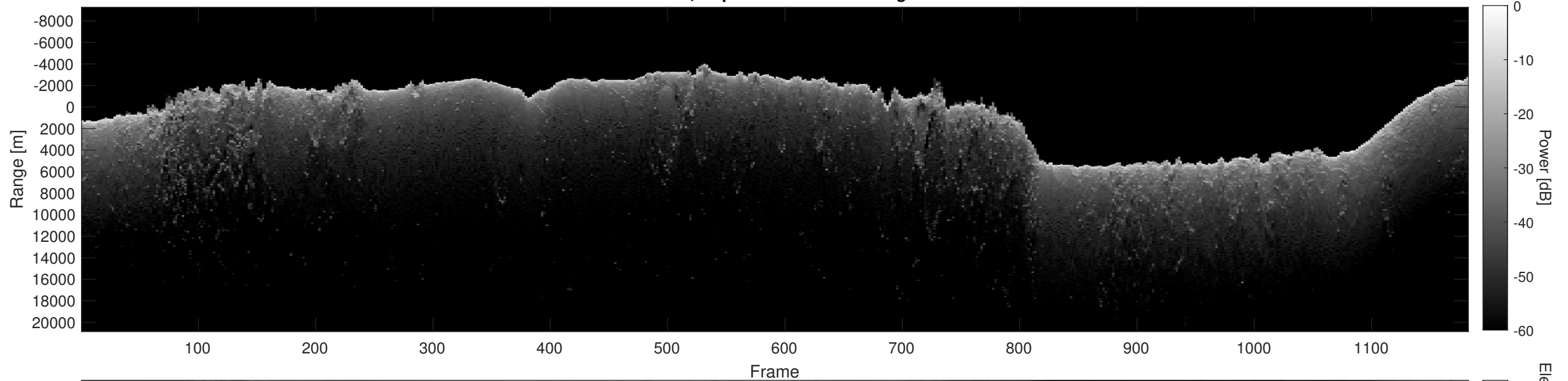
Orbit 9209, Depth-Corrected Cluttergram
