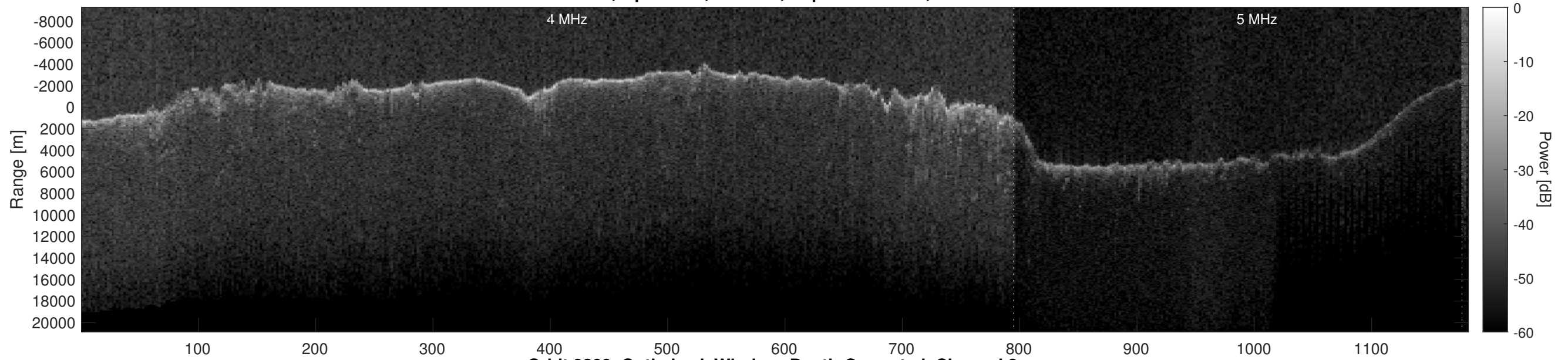
Orbit 9209, Optimized, Window, Depth-Corrected, Channel 2
