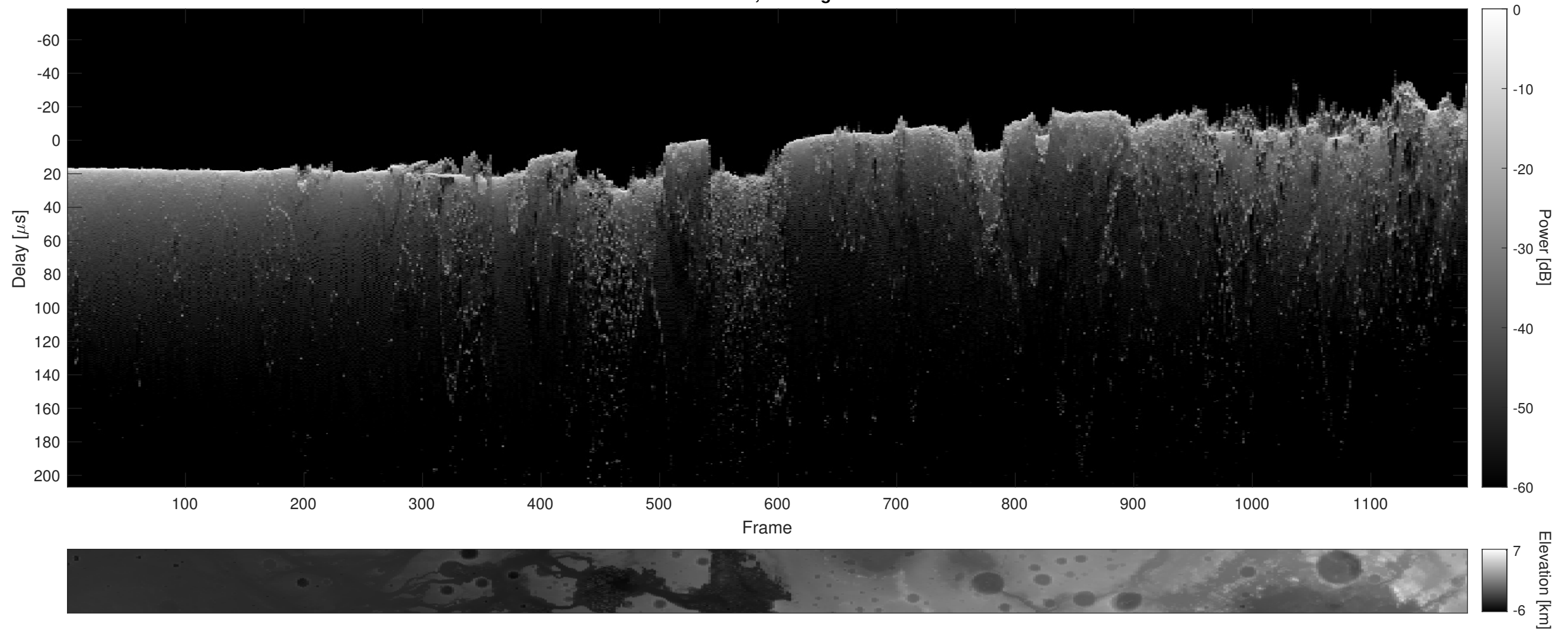
Orbit 9210, Cluttergram
