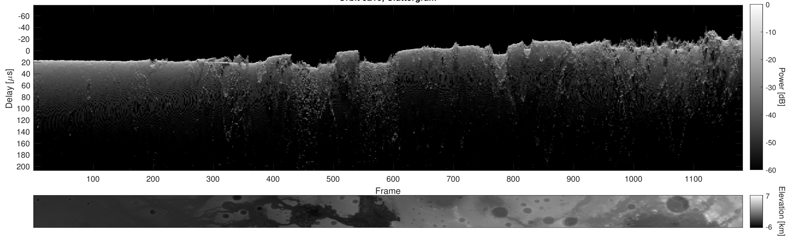
Orbit 9210, Cluttergram
