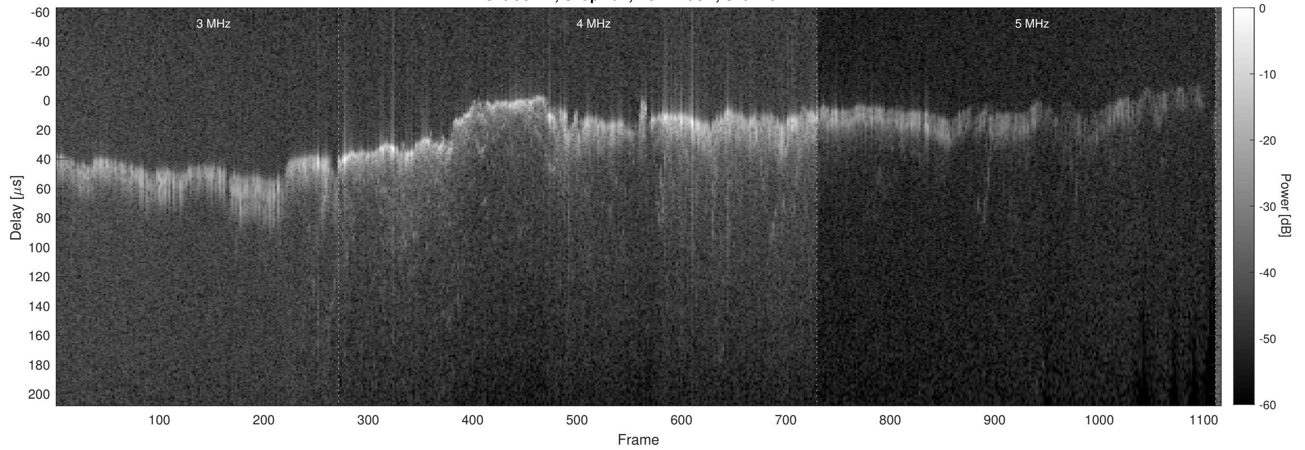
Orbit 9212, Chapman, No Window, Channel 2
