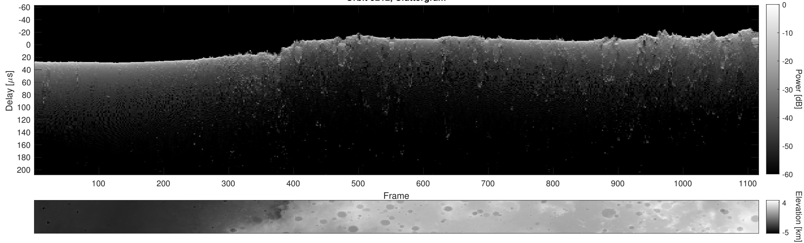
Orbit 9212, Cluttergram
