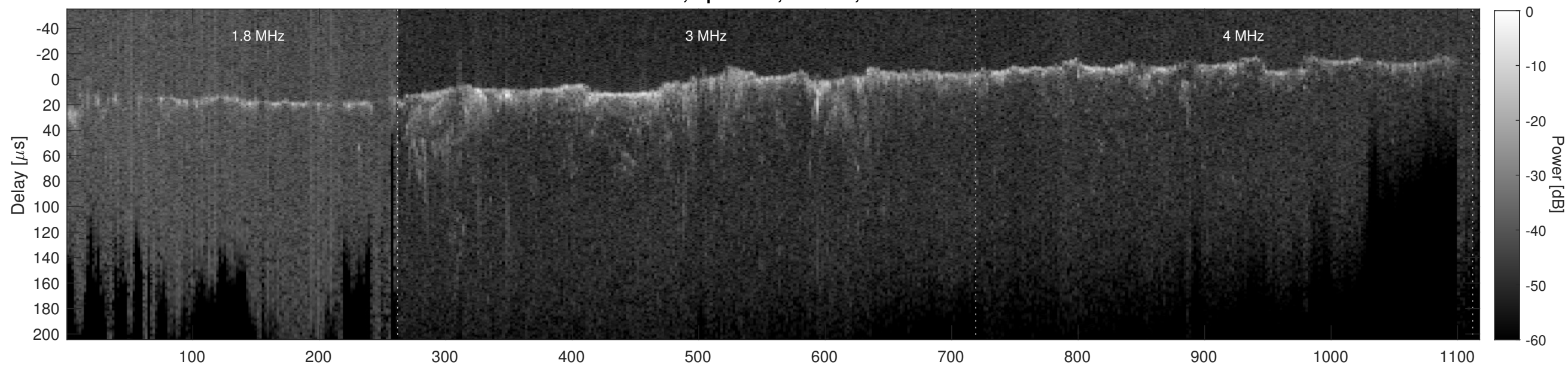
Orbit 9213, Cluttergram
