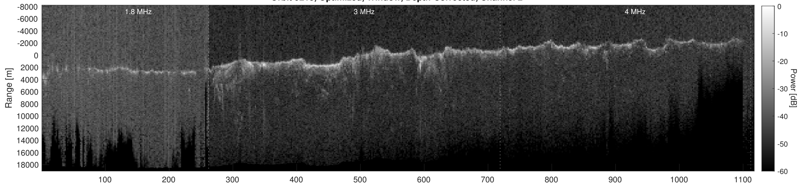
Orbit 9213, Depth-Corrected Cluttergram
