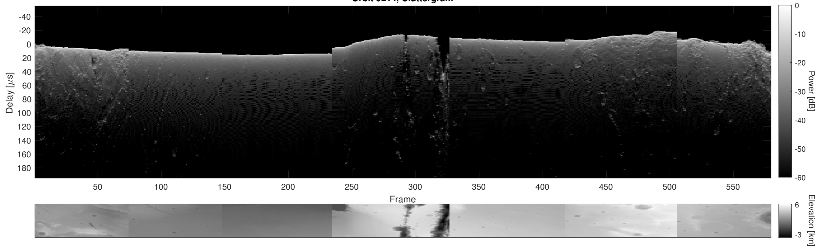
Orbit 9214, Cluttergram
