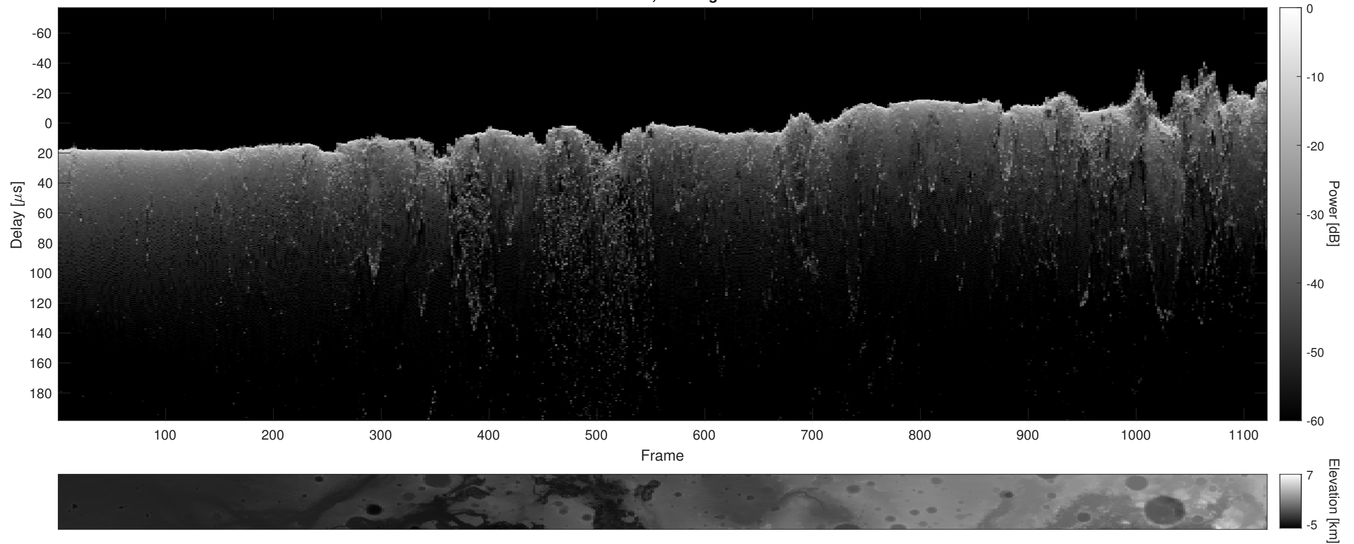
Orbit 9217, Cluttergram
