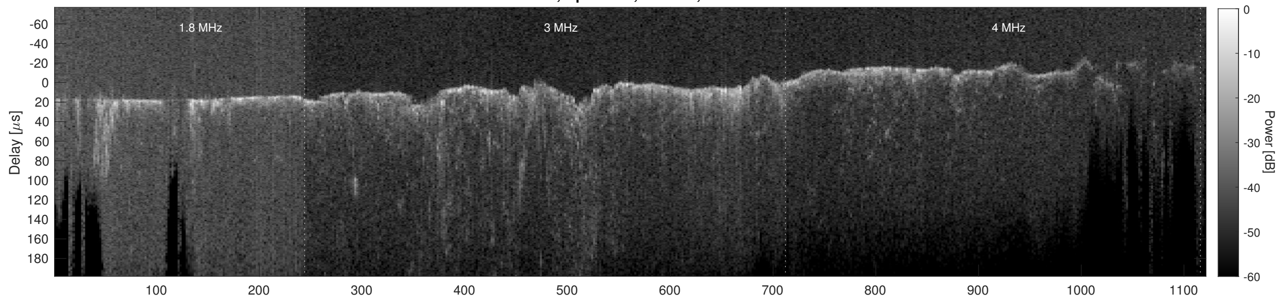
Orbit 9217, Cluttergram
