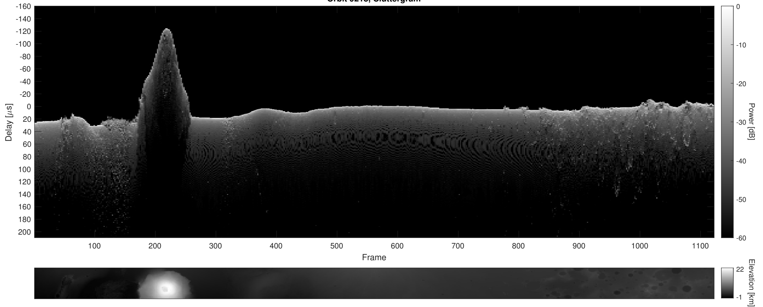
Orbit 9218, Cluttergram
