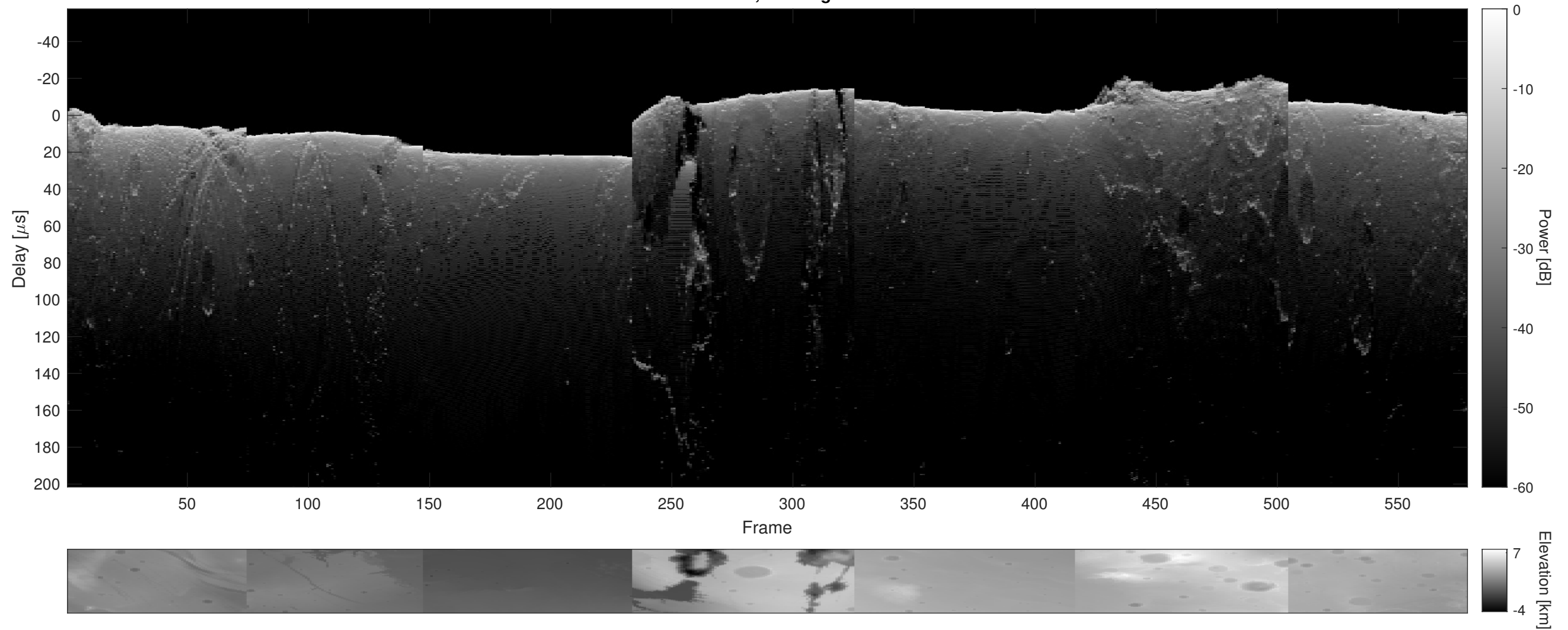
Orbit 9221, Cluttergram
