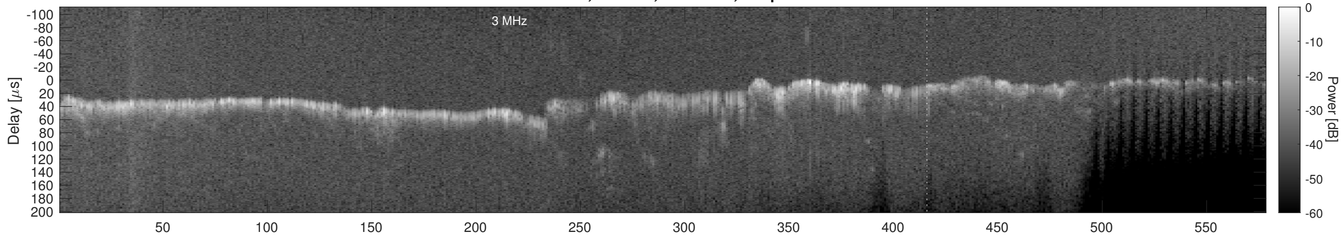
Orbit 9221, Window, Channel 2, Optimized
