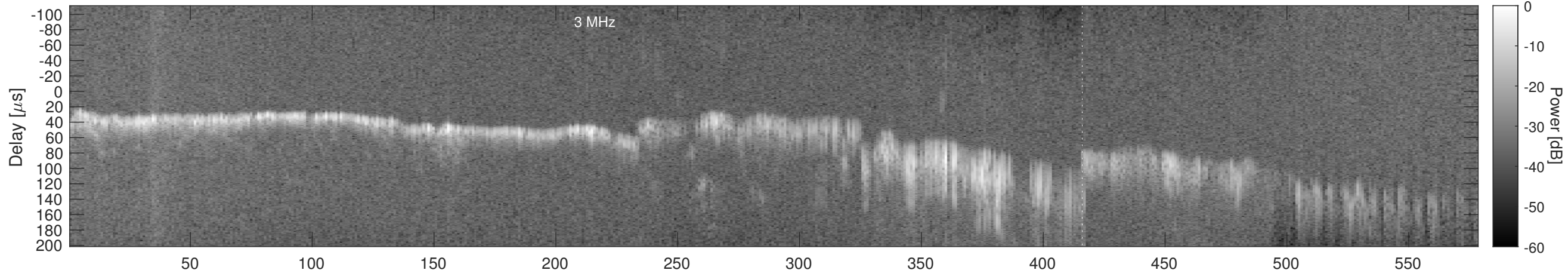
Orbit 9221, Window, Channel 2, Chapman
