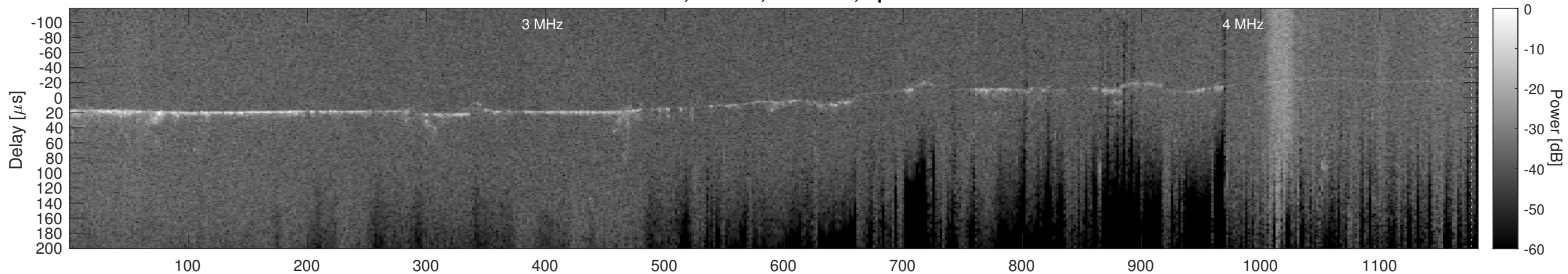
Orbit 9222, Cluttergram
