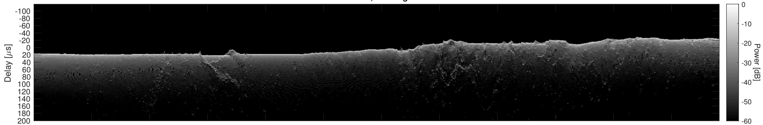
Orbit 9222, Cluttergram
