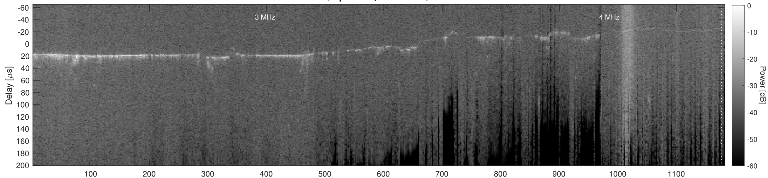
Orbit 9222, Cluttergram
