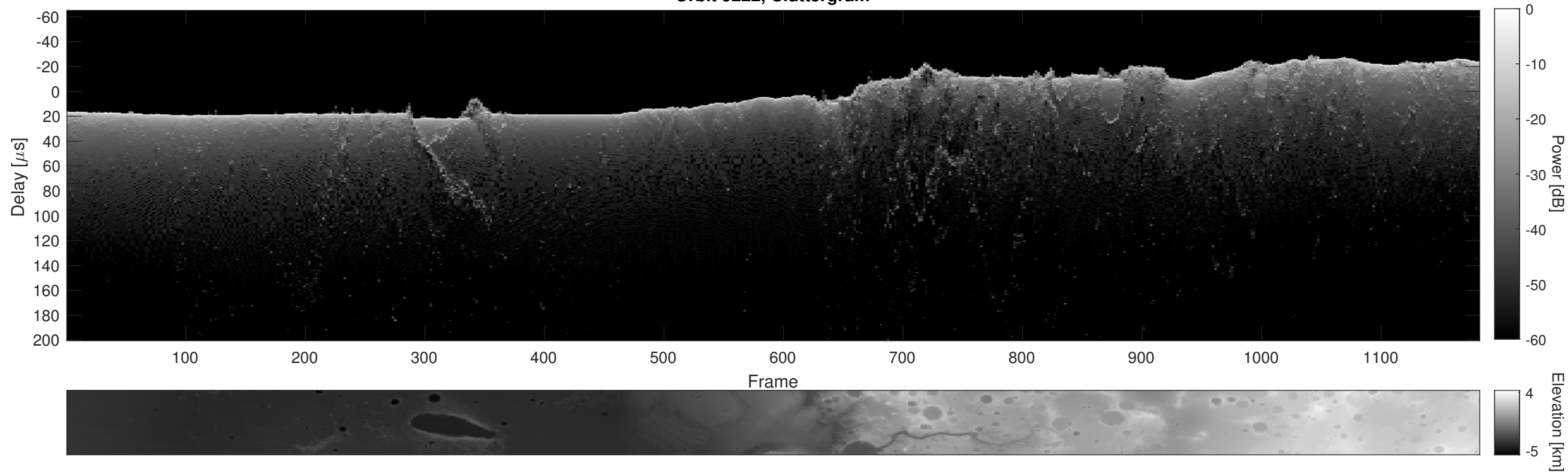
Orbit 9222, Cluttergram
