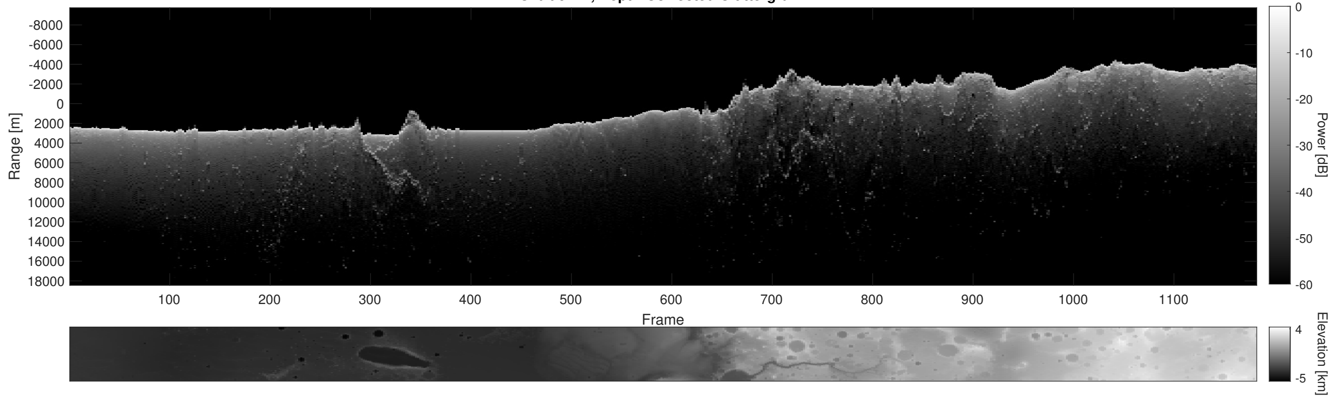
Orbit 9222, Depth-Corrected Cluttergram
