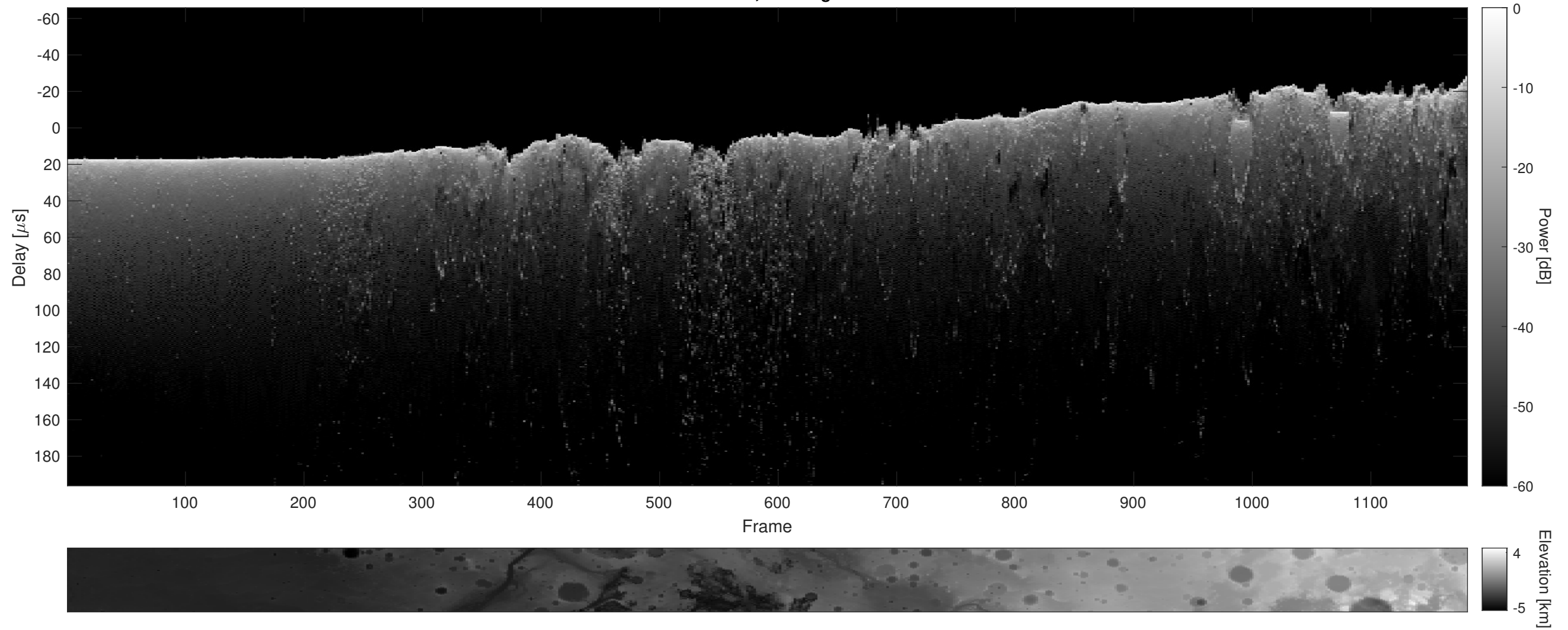
Orbit 9224, Cluttergram
