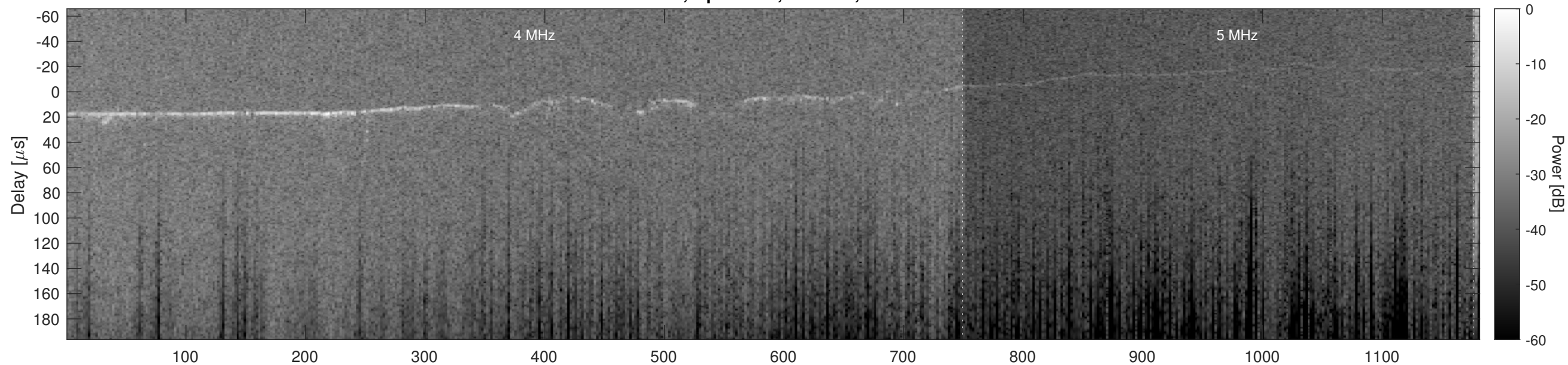
Orbit 9224, Optimized, Window, Channel 2
