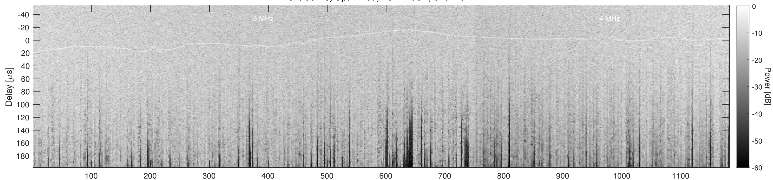
Orbit 9225, Cluttergram
