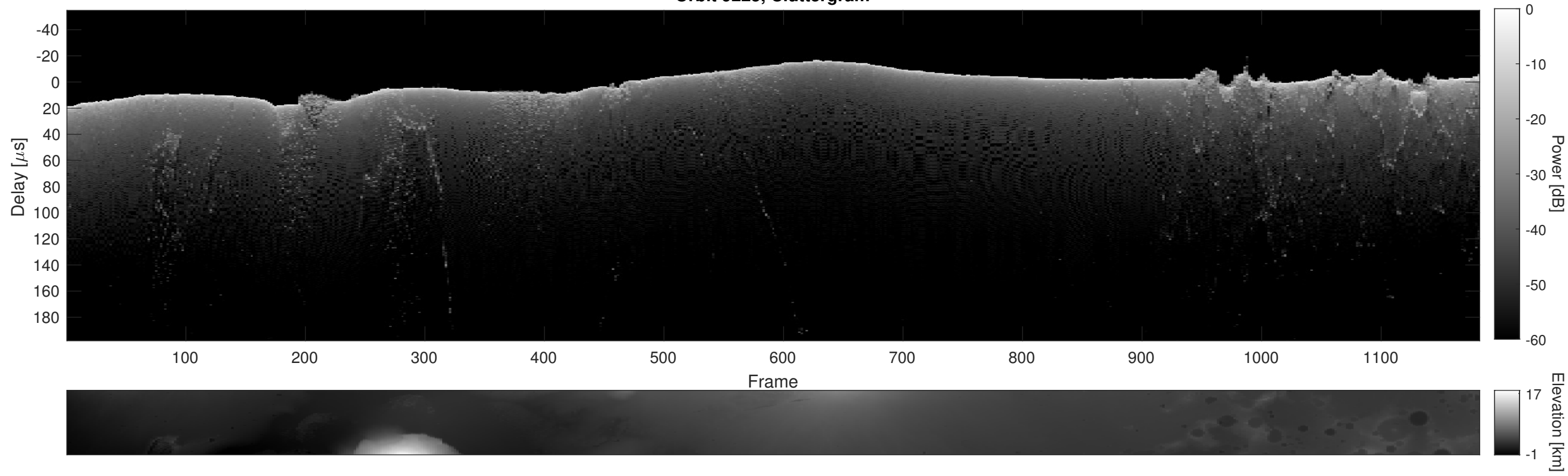
Orbit 9225, Cluttergram
