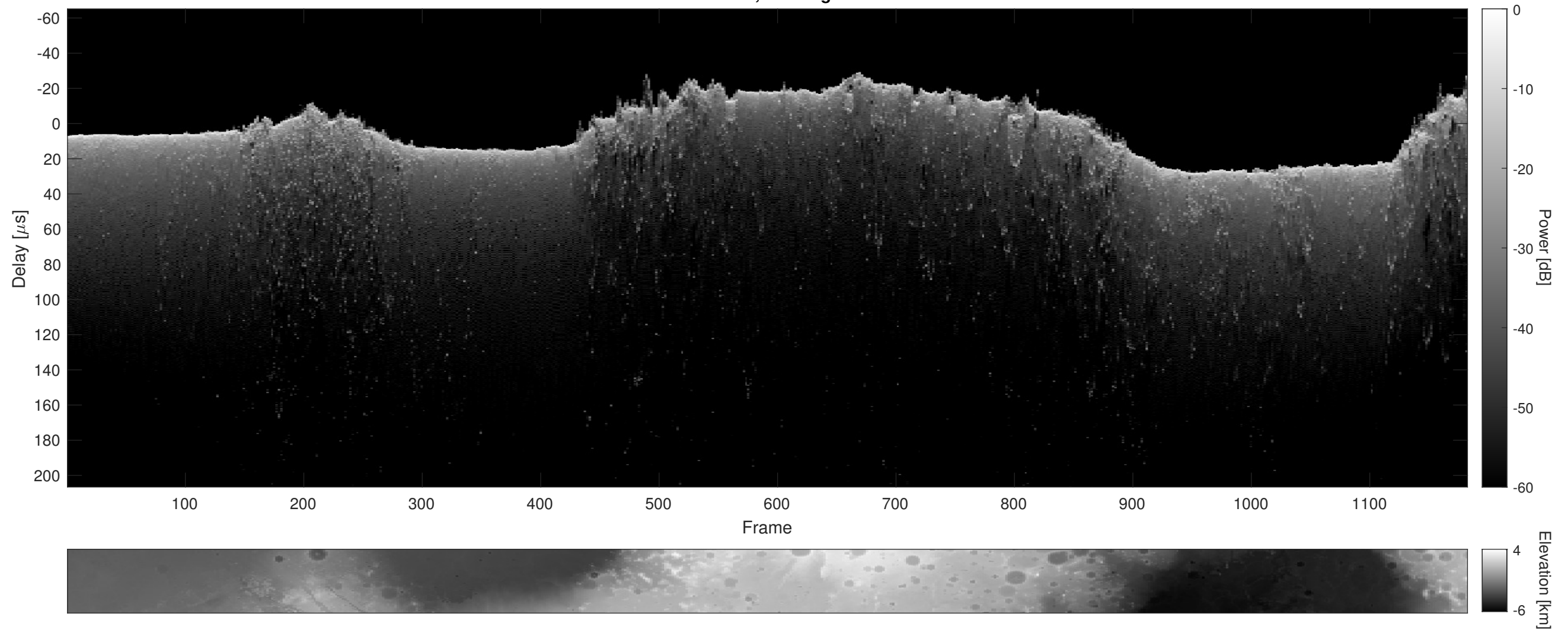
Orbit 9230, Cluttergram
