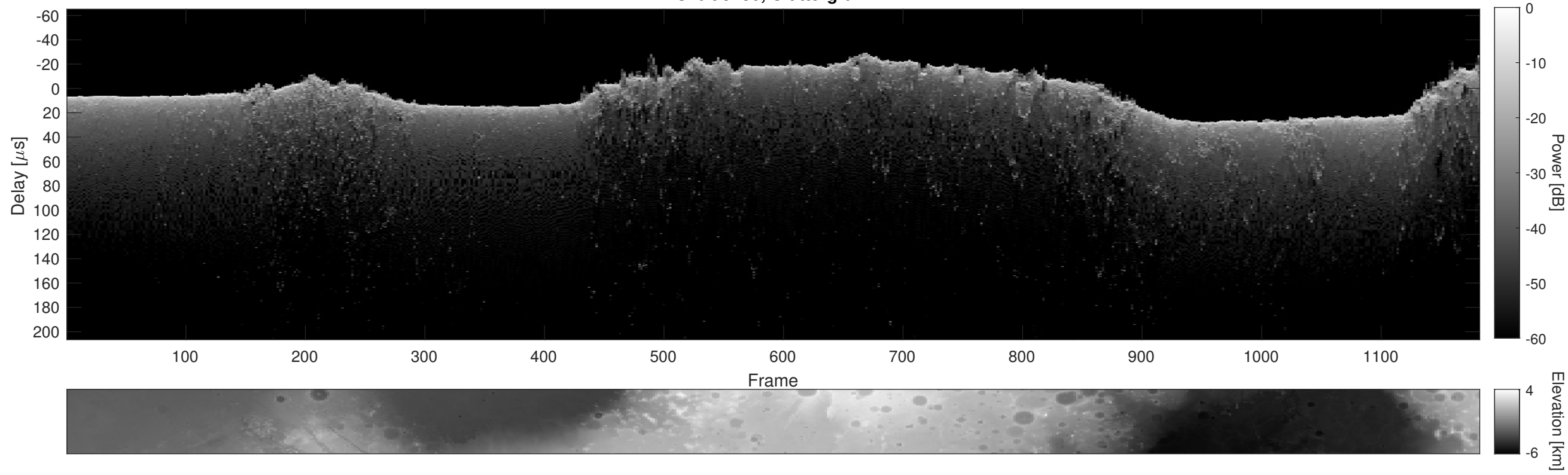
Orbit 9230, Cluttergram
