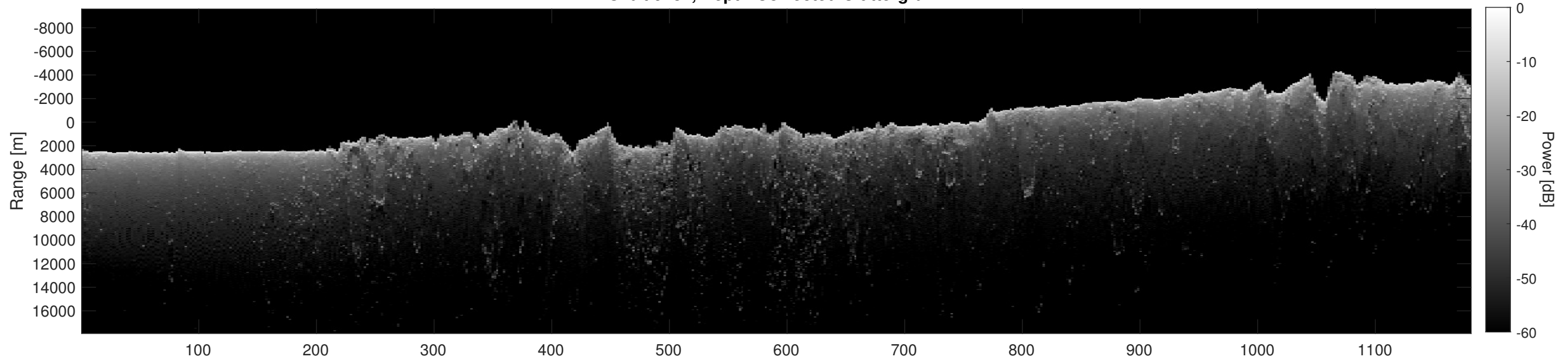
Orbit 9231, Depth-Corrected Cluttergram
