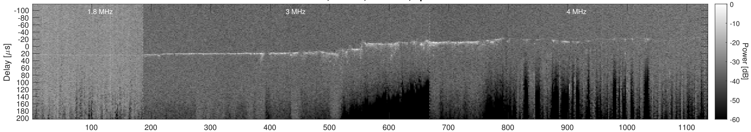
Orbit 9233, Cluttergram
