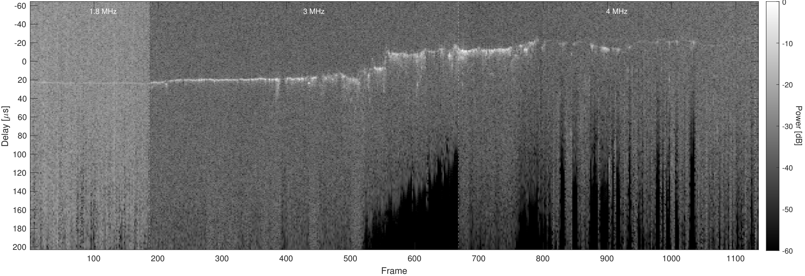
Orbit 9233, Optimized, No Window, Channel 2
