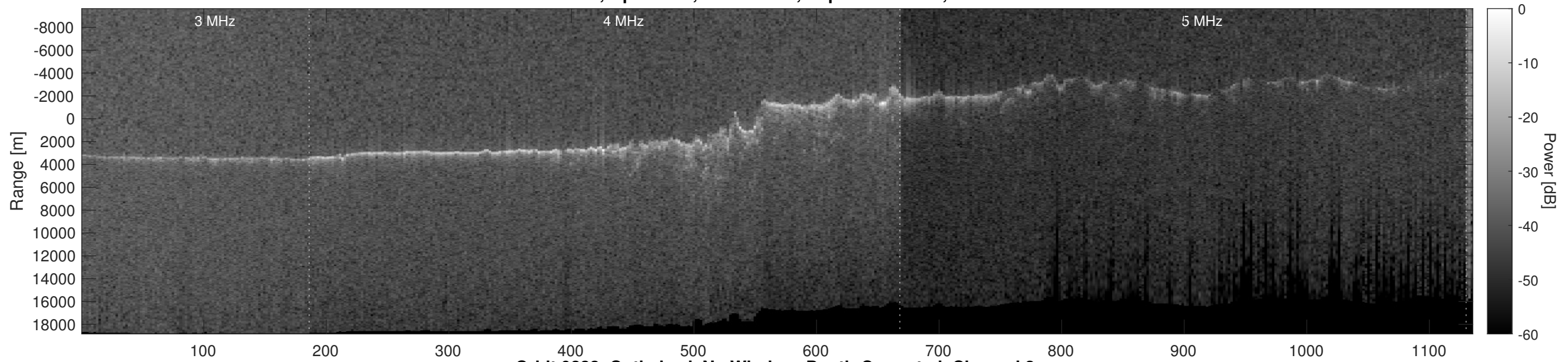
Orbit 9233, Optimized, No Window, Depth-Corrected, Channel 2
