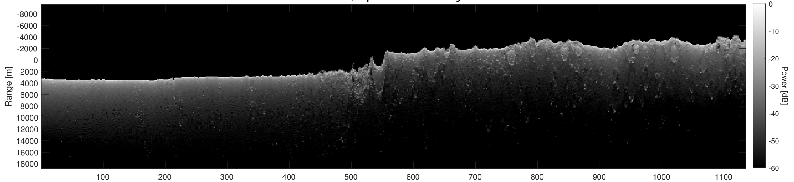
Orbit 9233, Depth-Corrected Cluttergram
