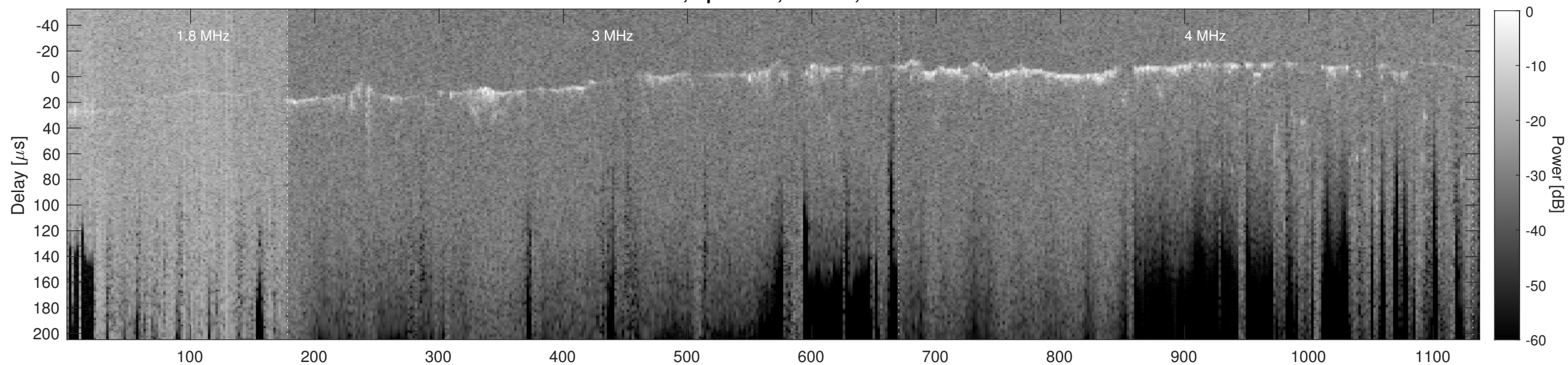
Orbit 9234, Cluttergram
