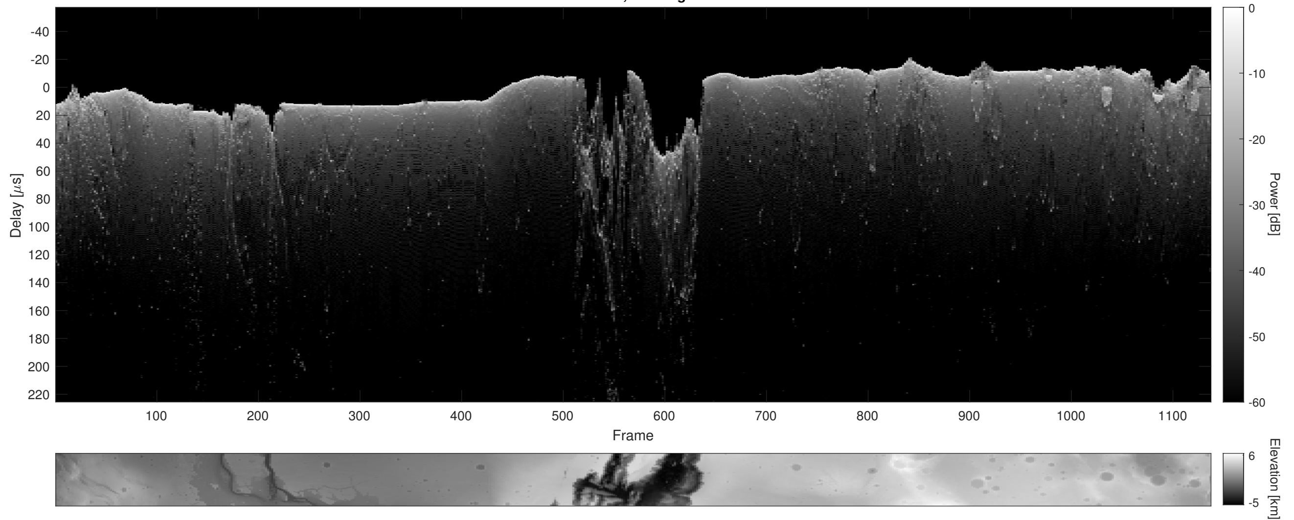
Orbit 9235, Cluttergram
