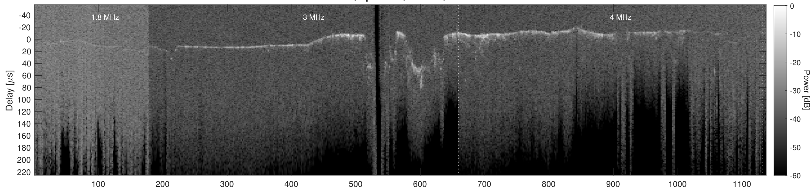
Orbit 9235, Cluttergram
