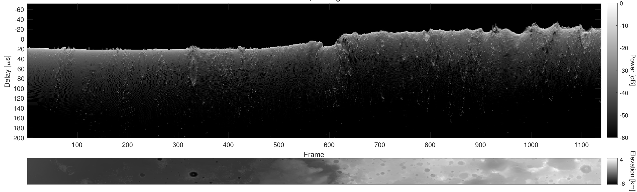
Orbit 9236, Cluttergram
