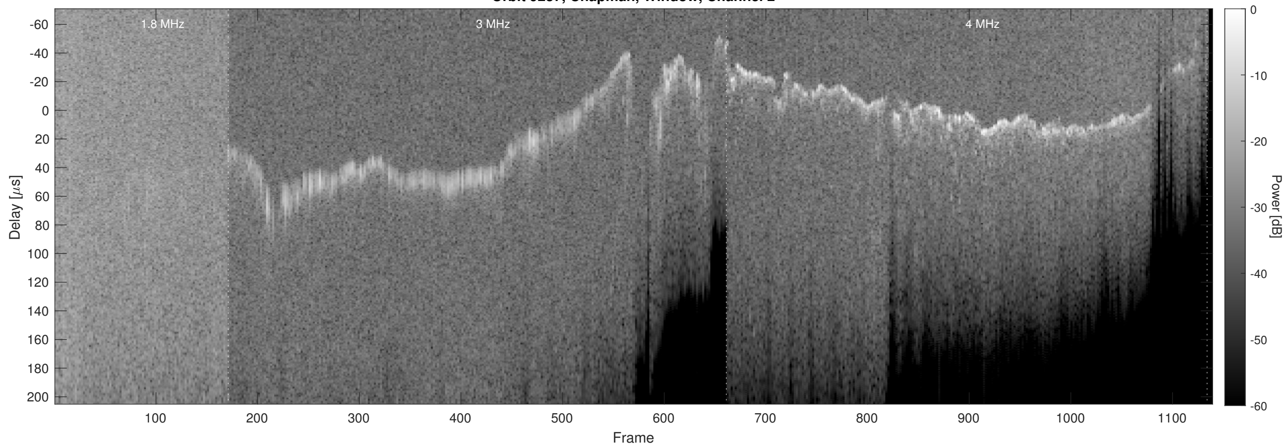
Orbit 9237, Chapman, Window, Channel 2
