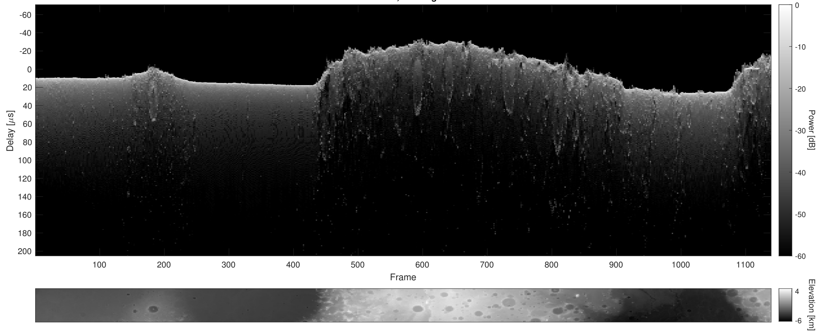
Orbit 9237, Cluttergram
