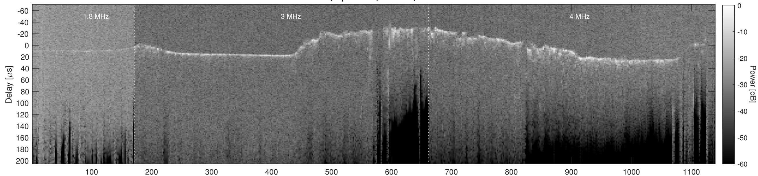
Orbit 9237, Cluttergram
