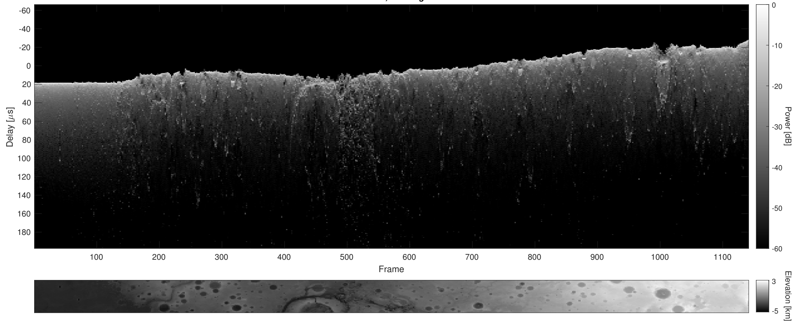
Orbit 9238, Cluttergram
