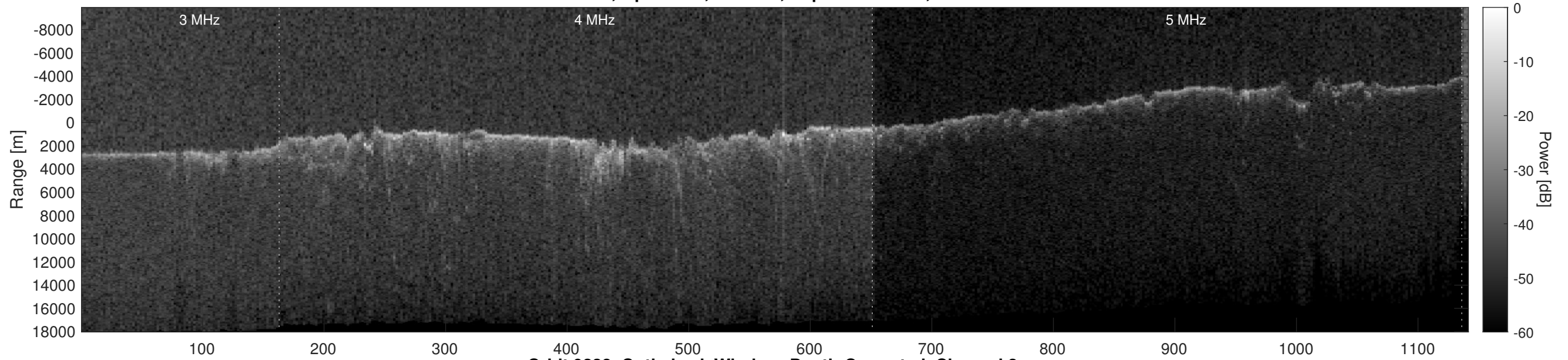
Orbit 9238, Optimized, Window, Depth-Corrected, Channel 2
